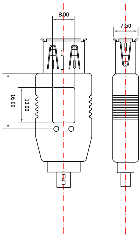
USB A FEMALE
