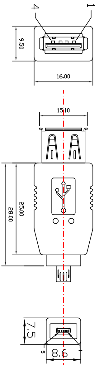
USB A FEMALE
