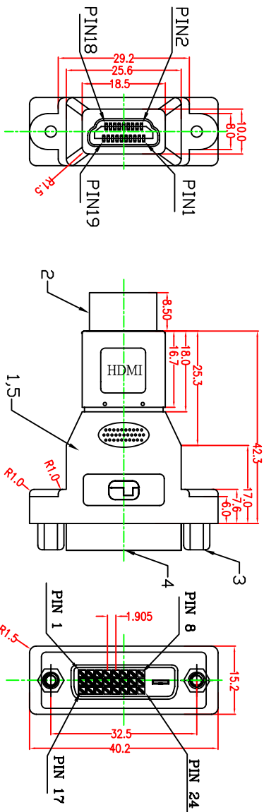
HDMI 19P MALE
