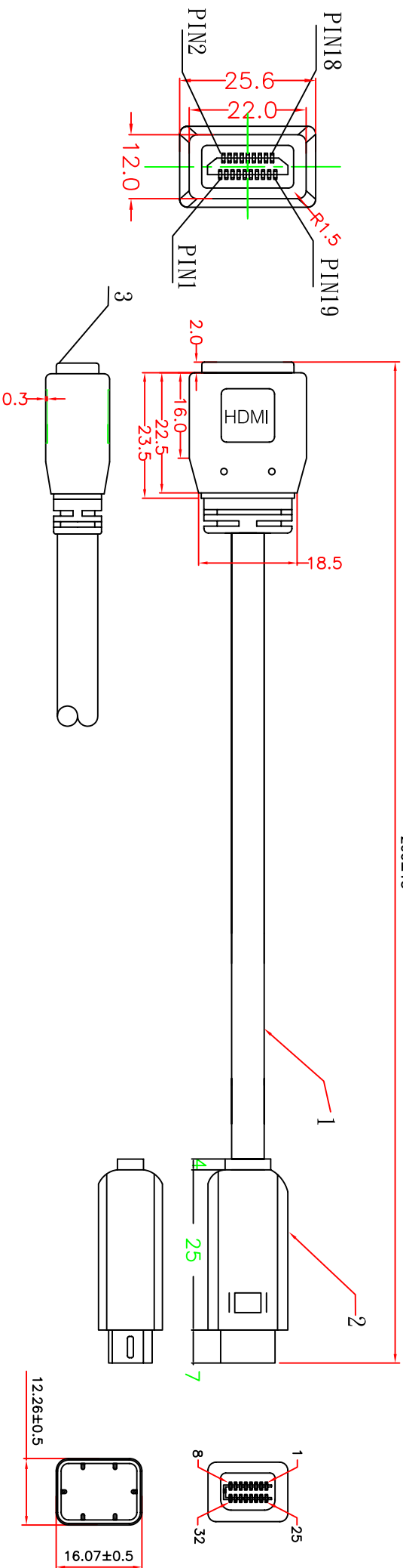
Pin Assignment HDMI19F MINI-DVI32P
