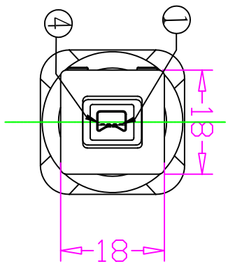
1394 4P MALE
