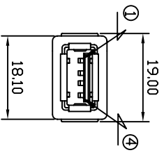
USB-A FEMALE
