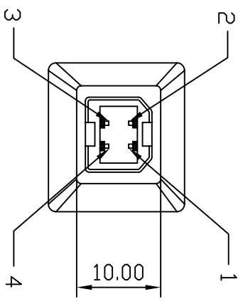
USB-B MALE
