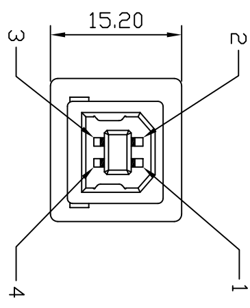
USB-B FEMALE
